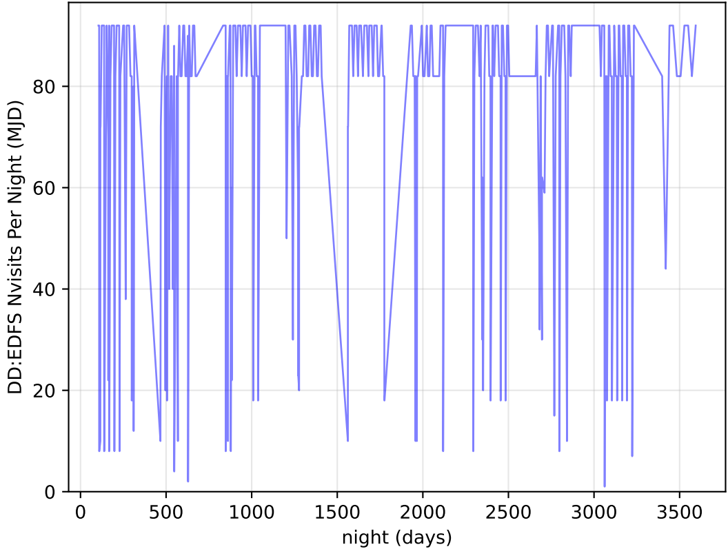
internal_u_expt38_nscale1.2v3.4_10yrs all bands: DD:EDFS Nvisits Per Night
