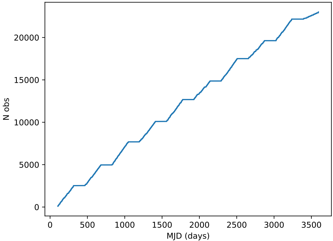
internal_u_expt38_nscale1.2v3.4_10yrs all bands: DD:EDFS Cumulative NVisits
