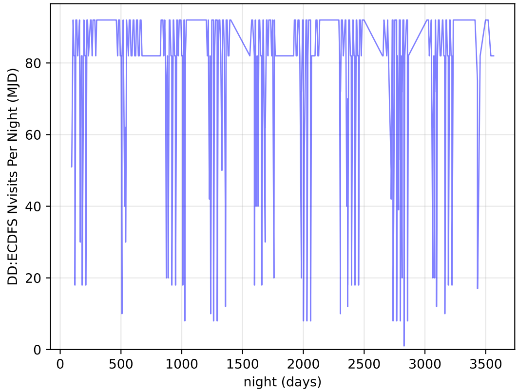
internal_u_expt38_nscale1.2v3.4_10yrs all bands: DD:ECDFS Nvisits Per Night
