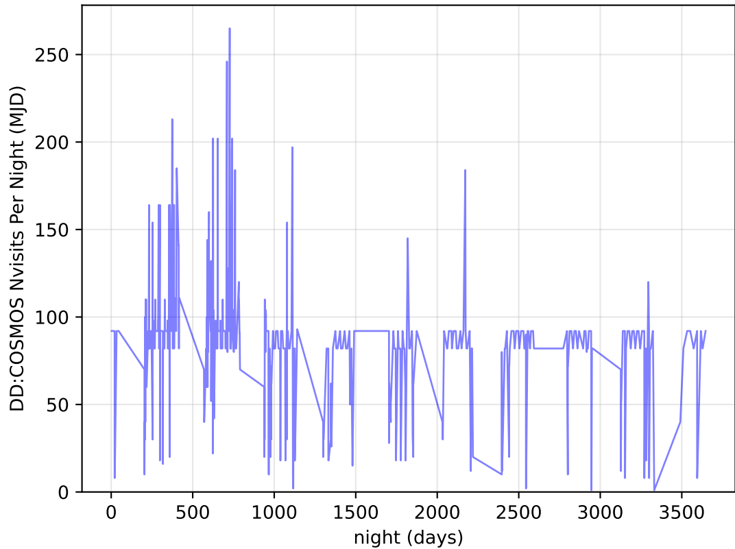
internal_u_expt38_nscale1.2v3.4_10yrs all bands: DD: COSMOS Nvisits Per Night
