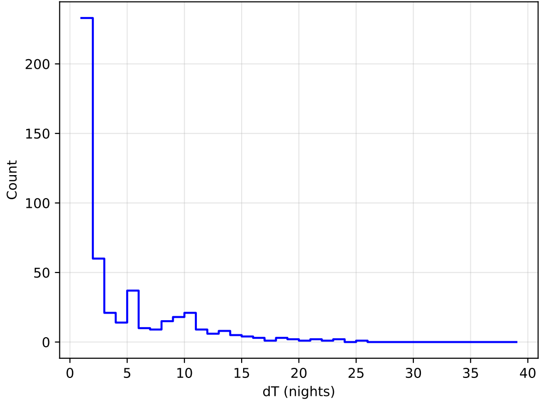
internal_u_expt38_nscale1.2v3.4_10yrs all bands: DD:COSMOS Delta Nights Histogram
