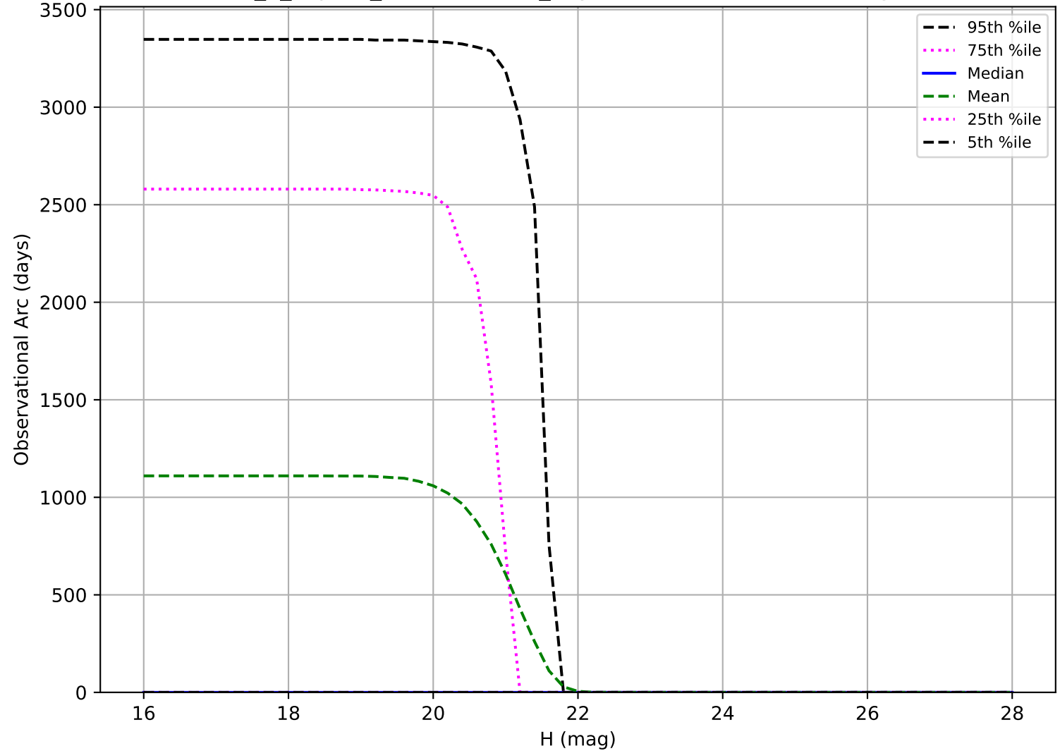
internal_u_expt38_nscale1.1v3.4_10yrs: Observational Arc Length Vatra
