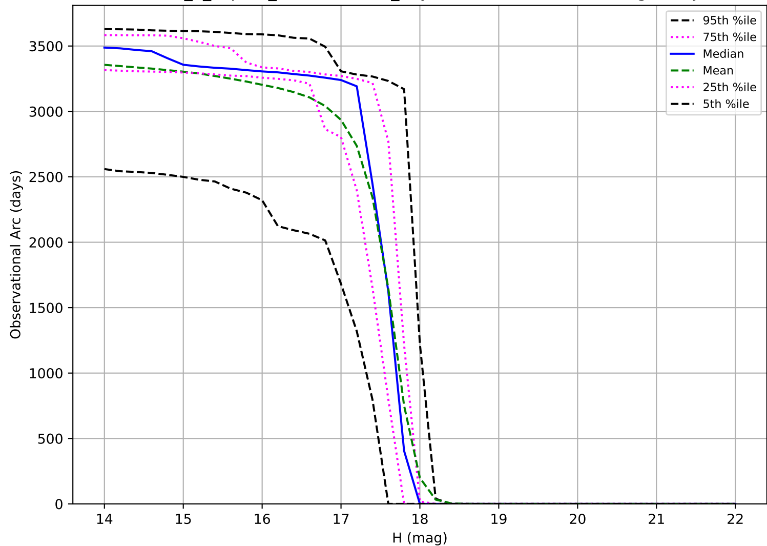
internal_u_expt38_nscale1.1v3.4_10yrs: Observational Arc Length Trojan
