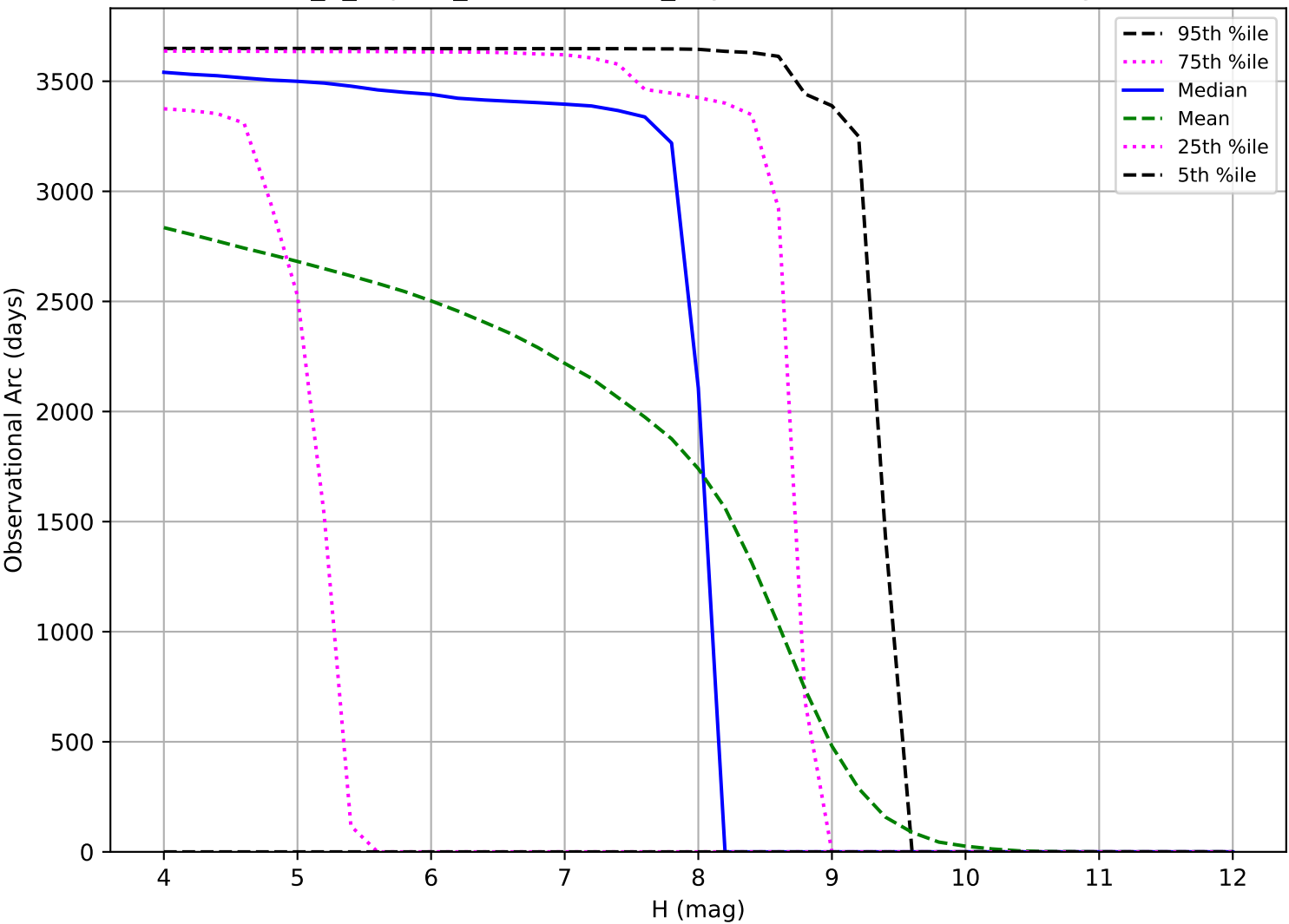
internal_u_expt38_nscale1.1v3.4_10yrs: Observational Arc Length TNO
