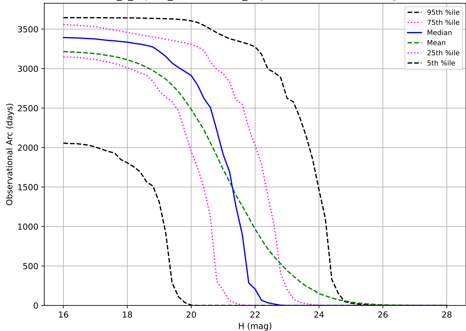
internal_u_expt38_nscale1.1v3.4_10yrs: Observational Arc Length PHA
