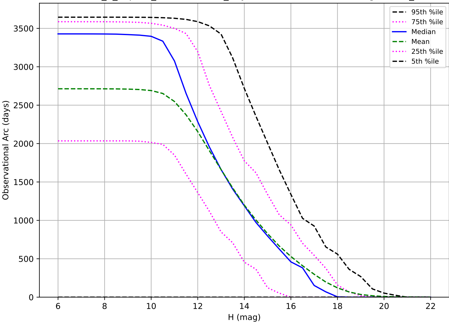
internal_u_expt38_nscale1.1v3.4_10yrs: Observational Arc Length OCC_r5
