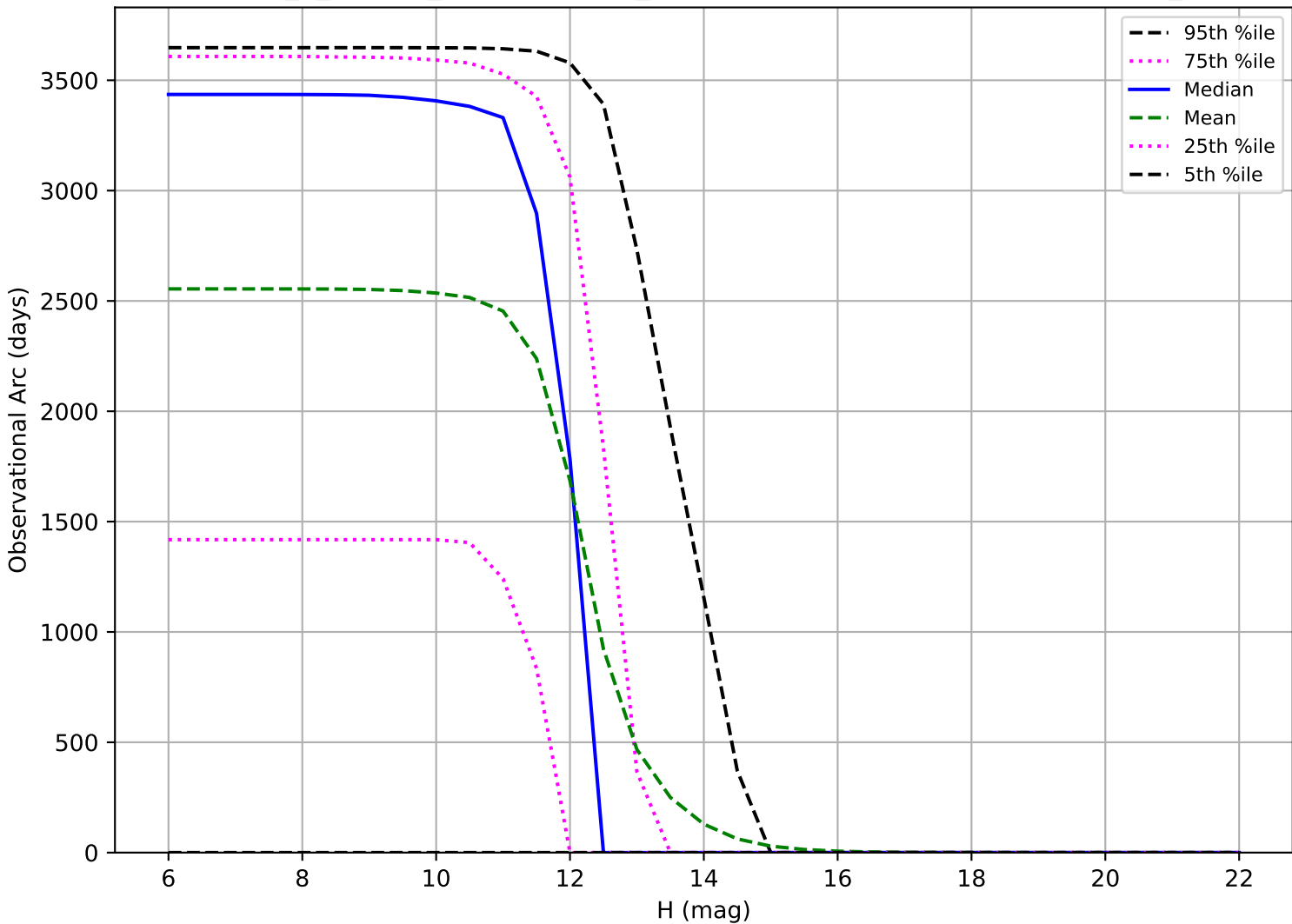
internal_u_expt38_nscale1.1v3.4_10yrs: Observational Arc Length OCC_r20
