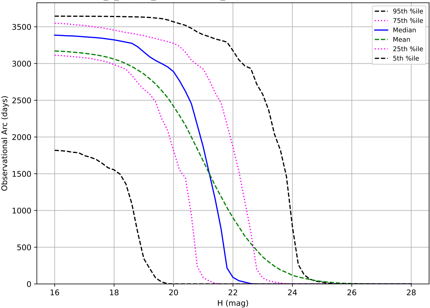
internal_u_expt38_nscale1.1v3.4_10yrs: Observational Arc Length NEO
