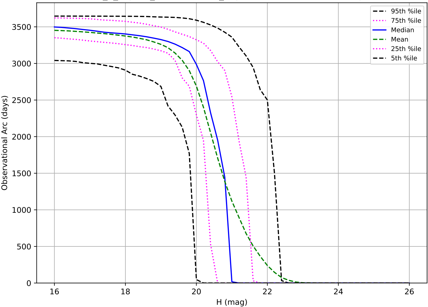
internal_u_expt38_nscale1.1v3.4_10yrs: Observational Arc Length MBA
