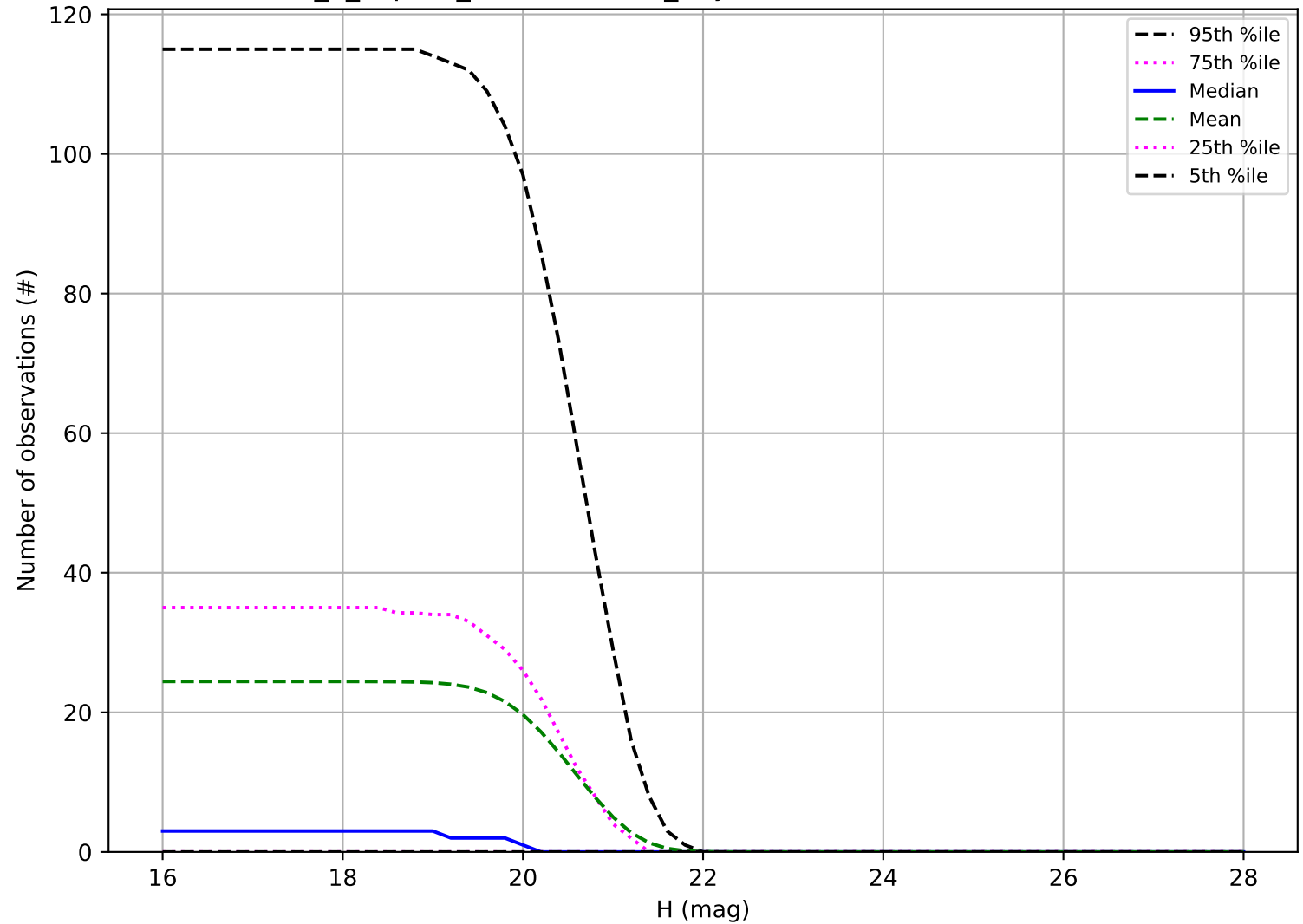
internal_u_expt38_nscale1.1v3.4_10yrs: Number of observations Vatira
