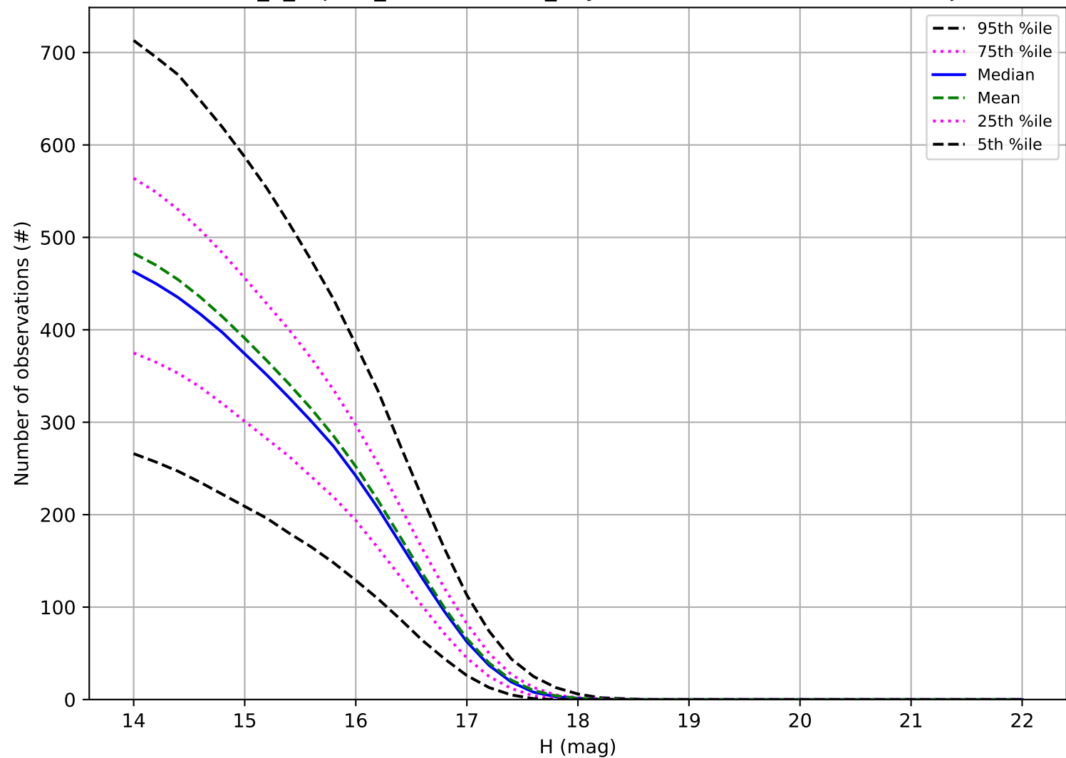
internal_u_expt38_nscale1.1v3.4_10yrs: Number of observations Trojan
