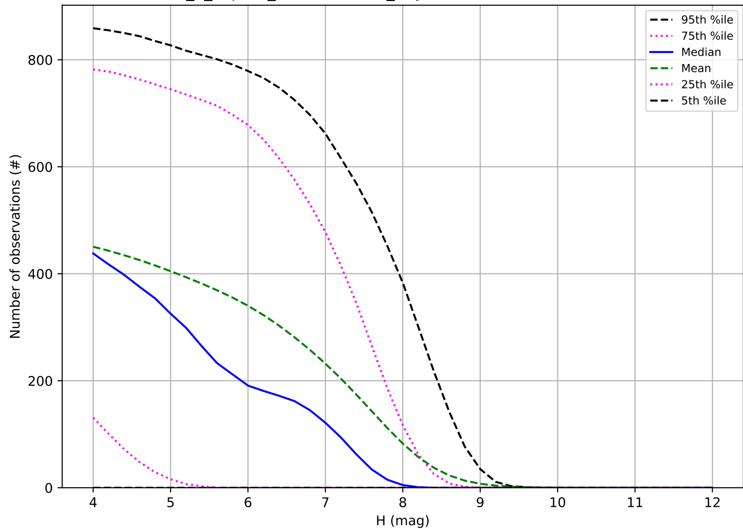
internal_u_expt38_nscale1.1v3.4_10yrs: Number of observations TNO
