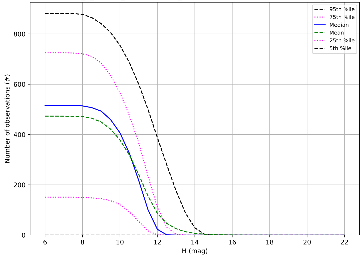
internal_u_expt38_nscale1.1v3.4_10yrs: Number of observations OCC_r20
