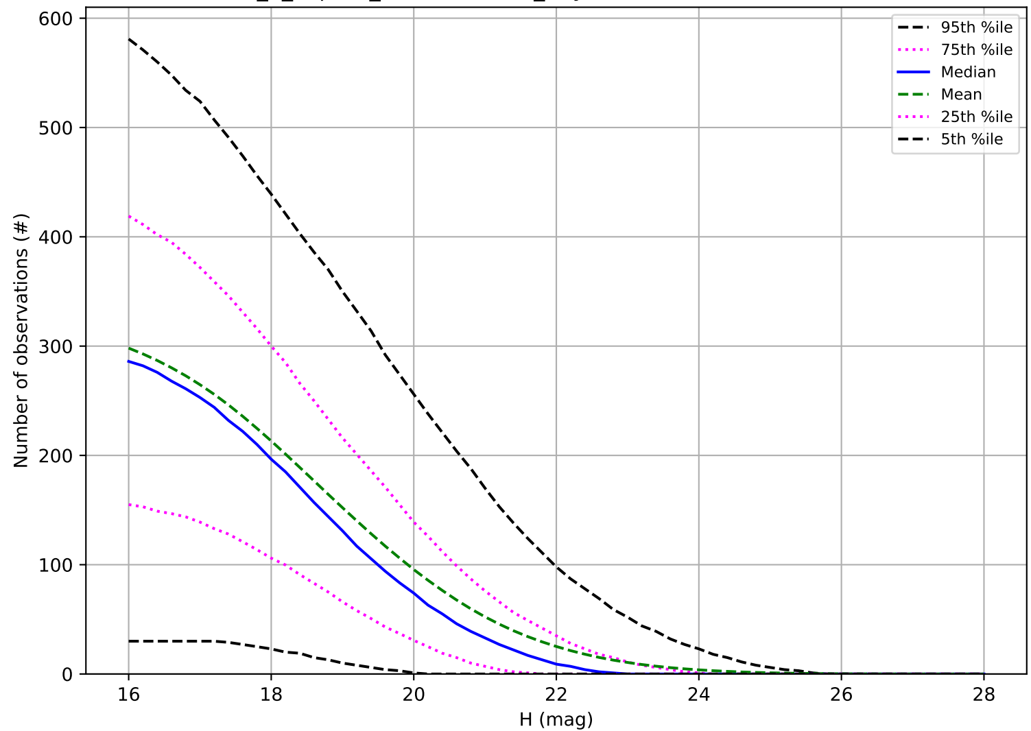
internal_u_expt38_nscale1.1v3.4_10yrs: Number of observations NEO
