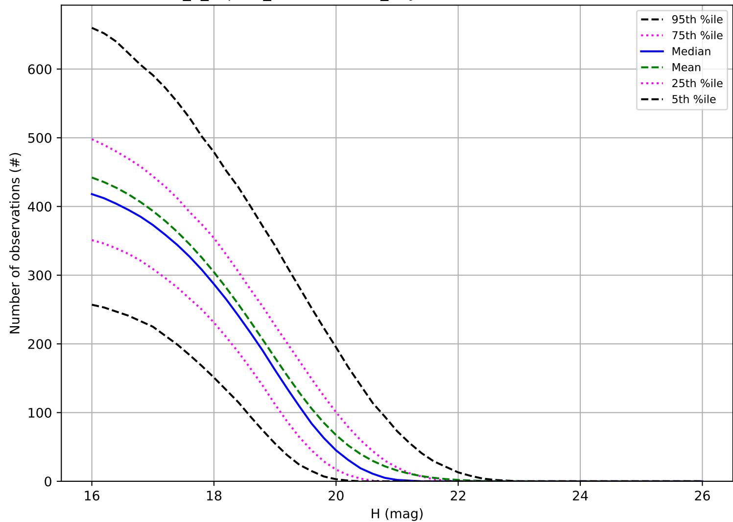
internal_u_expt38_nscale1.1v3.4_10yrs: Number of observations MBA
