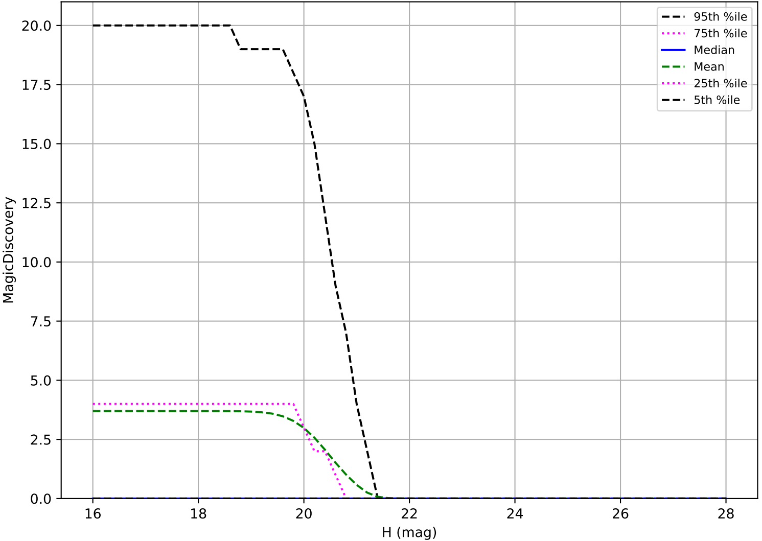
internal_u_expt38_nscale1.1v3.4_10yrs: Vatira 6 detections in 60 nights detection loss
