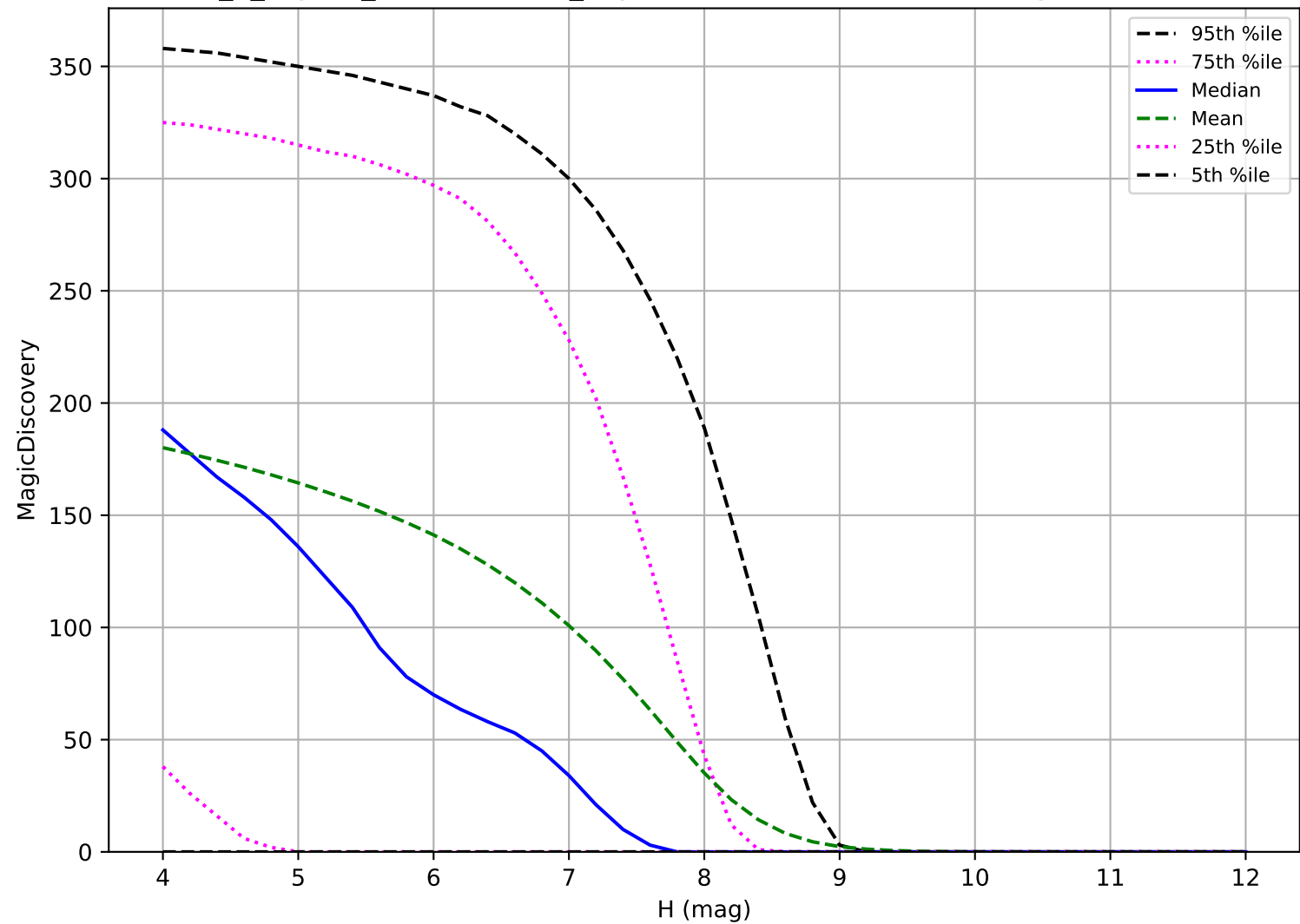
internal_u_expt38_nscale1.1v3.4_10yrs: TNO 6 detections in 60 nights detection loss
