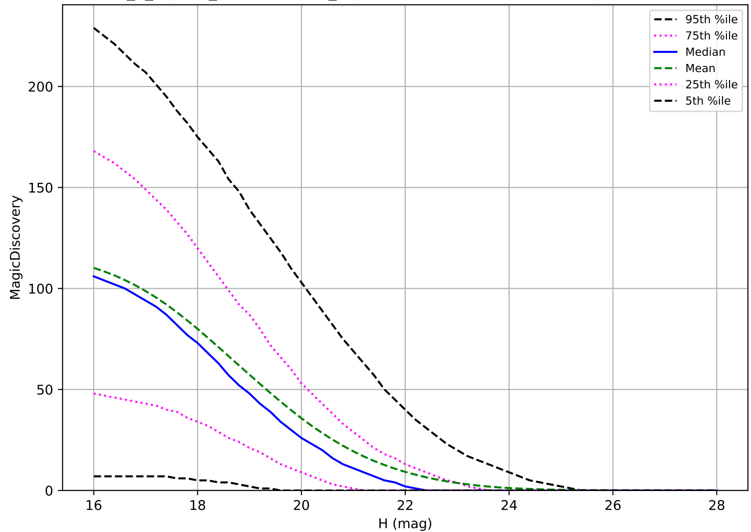
internal_u_expt38_nscale1.1v3.4_10yrs: PHA 6 detections in 60 nights detection loss
