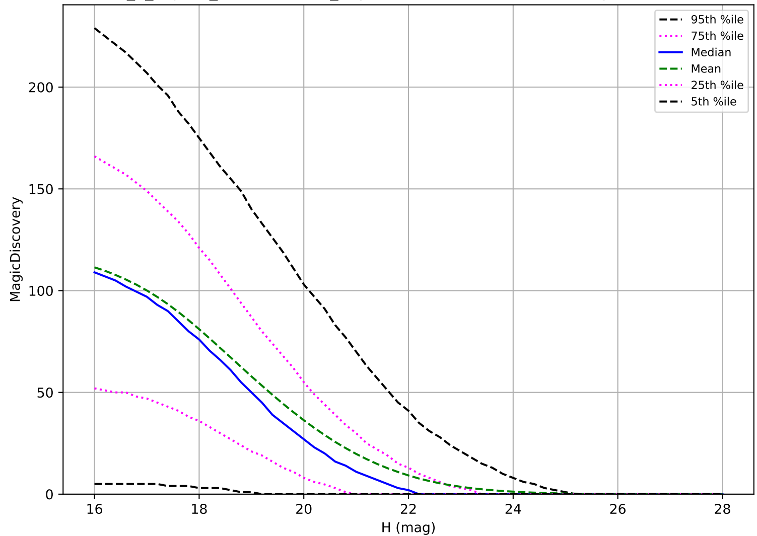
internal_u_expt38_nscale1.1v3.4_10yrs: NEO 6 detections in 60 nights detection loss
