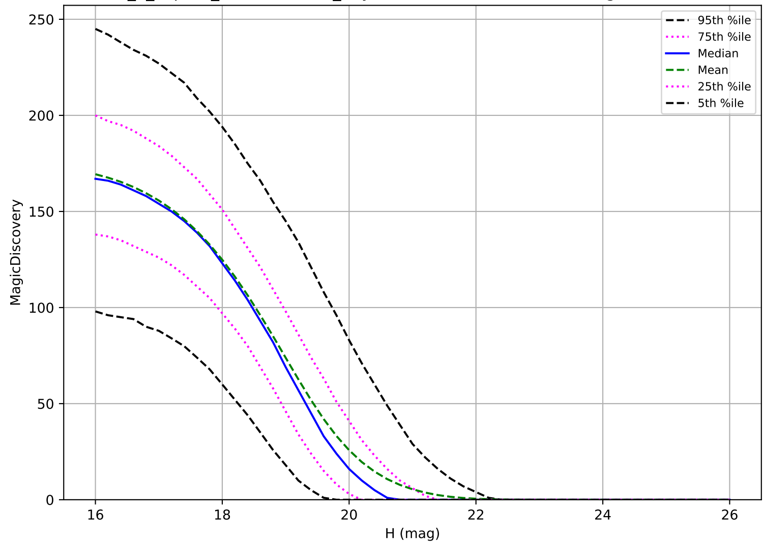
internal_u_expt38_nscale1.1v3.4_10yrs: MBA 6 detections in 60 nights detection loss
