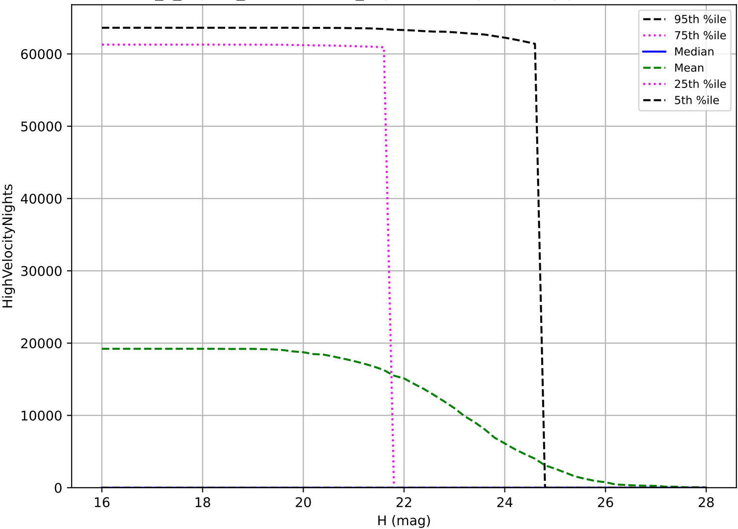
internal_u_expt38_nscale1.1v3.4_10yrs: NEO High velocity pair detection loss
