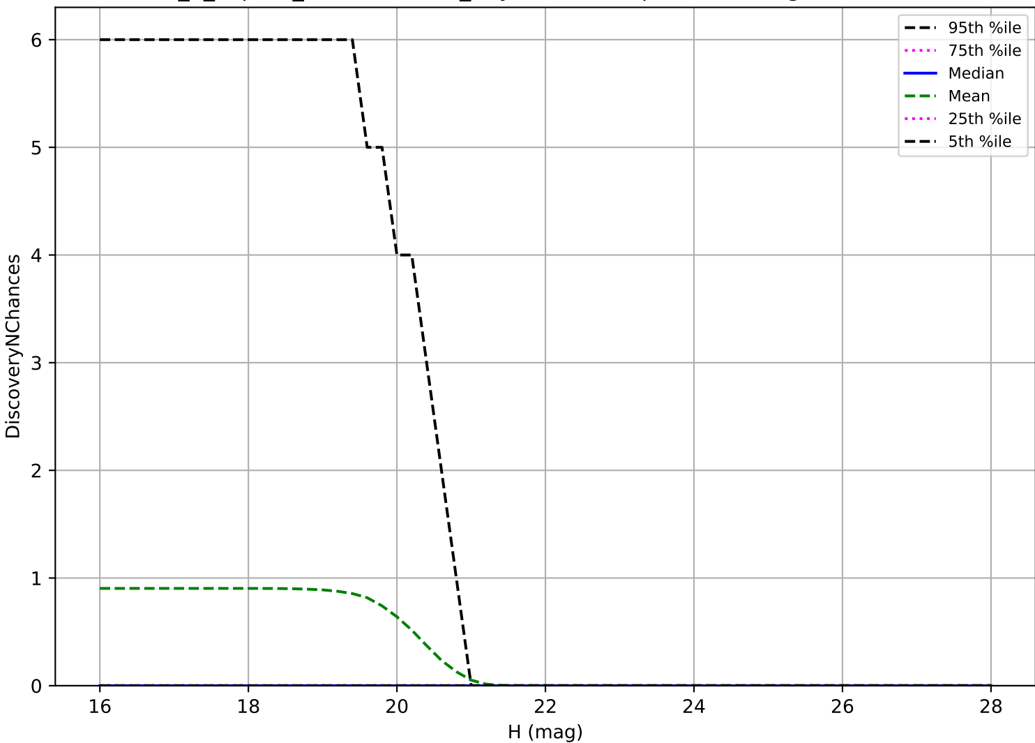
internal_u_expt38_nscale1.1v3.4_10yrs: Vatira 3 pairs in 15 nights detection loss
