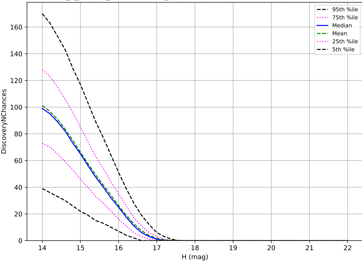
internal_u_expt38_nscale1.1v3.4_10yrs: Trojan 3 pairs in 15 nights detection loss
