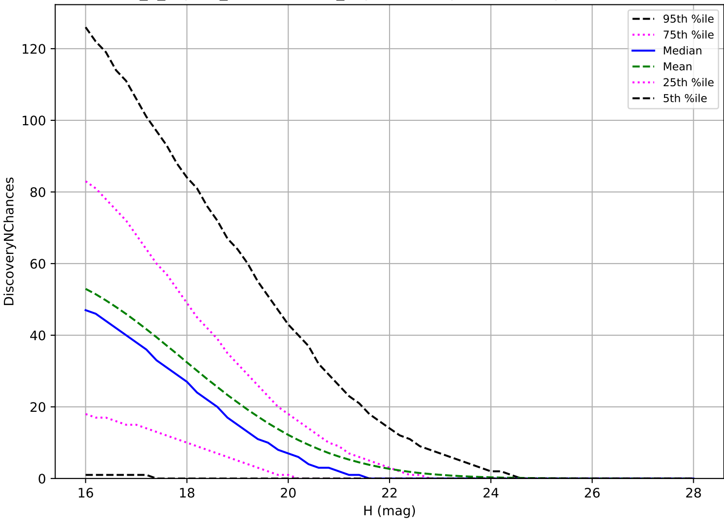
internal_u_expt38_nscale1.1v3.4_10yrs: PHA 3 pairs in 15 nights detection loss
