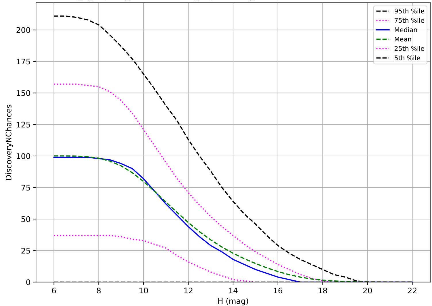
internal_u_expt38_nscale1.1v3.4_10yrs: OCC_r5 3 pairs in 15 nights detection loss
