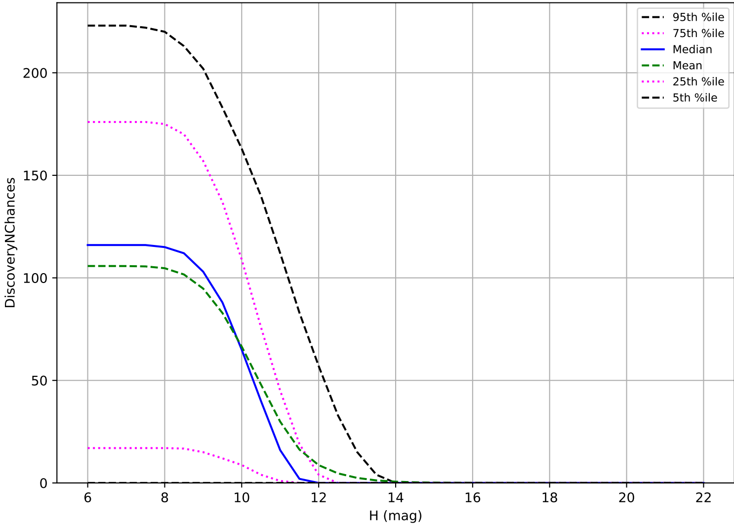
internal_u_expt38_nscale1.1v3.4_10yrs: OCC_r20 3 pairs in 15 nights detection loss
