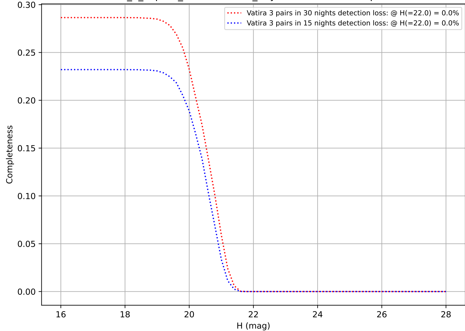
internal_u_expt38_nscale1.1v3.4_10yrs: DifferentialCompleteness
