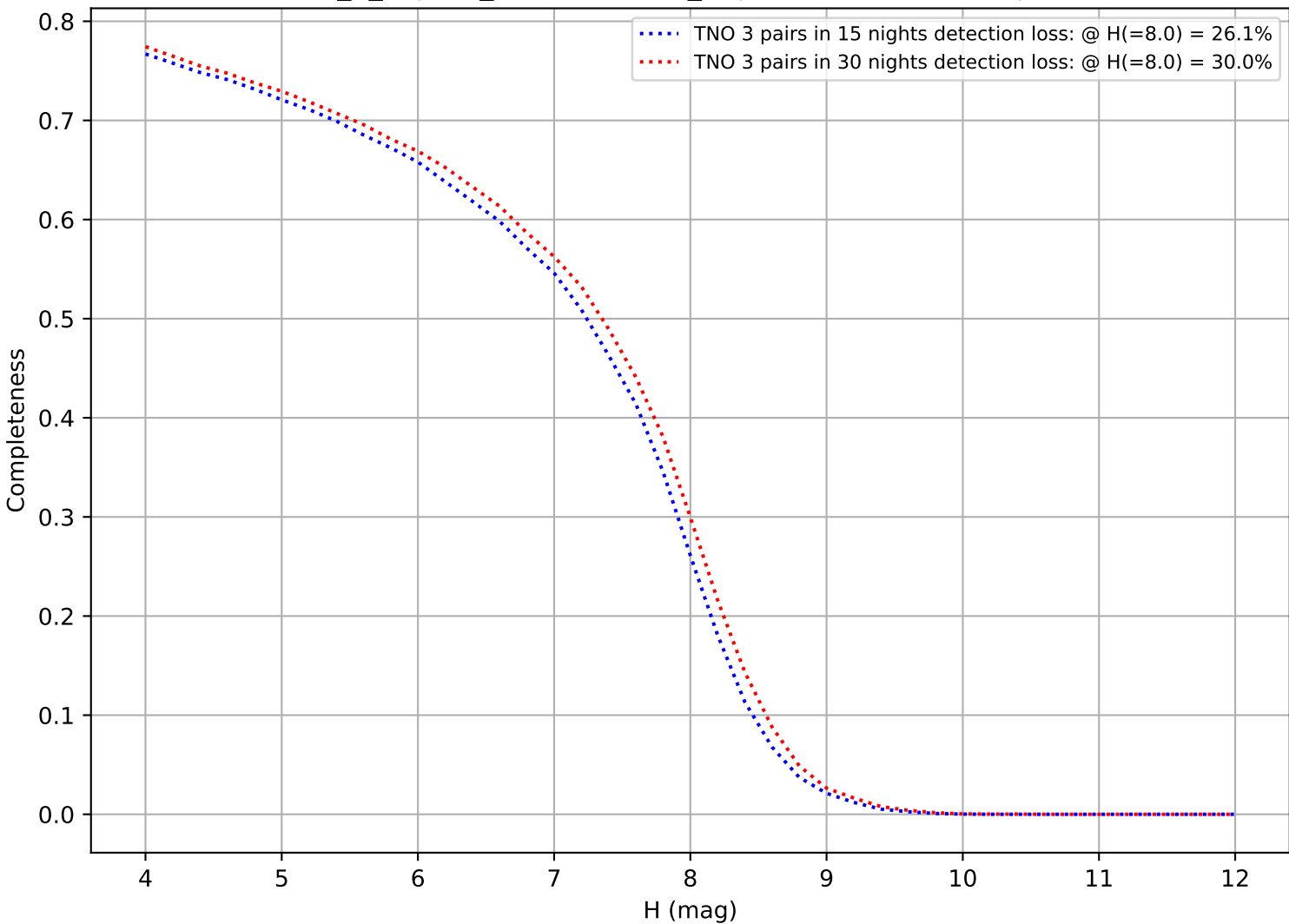
internal_u_expt38_nscale1.1v3.4_10yrs: DifferentialCompleteness
