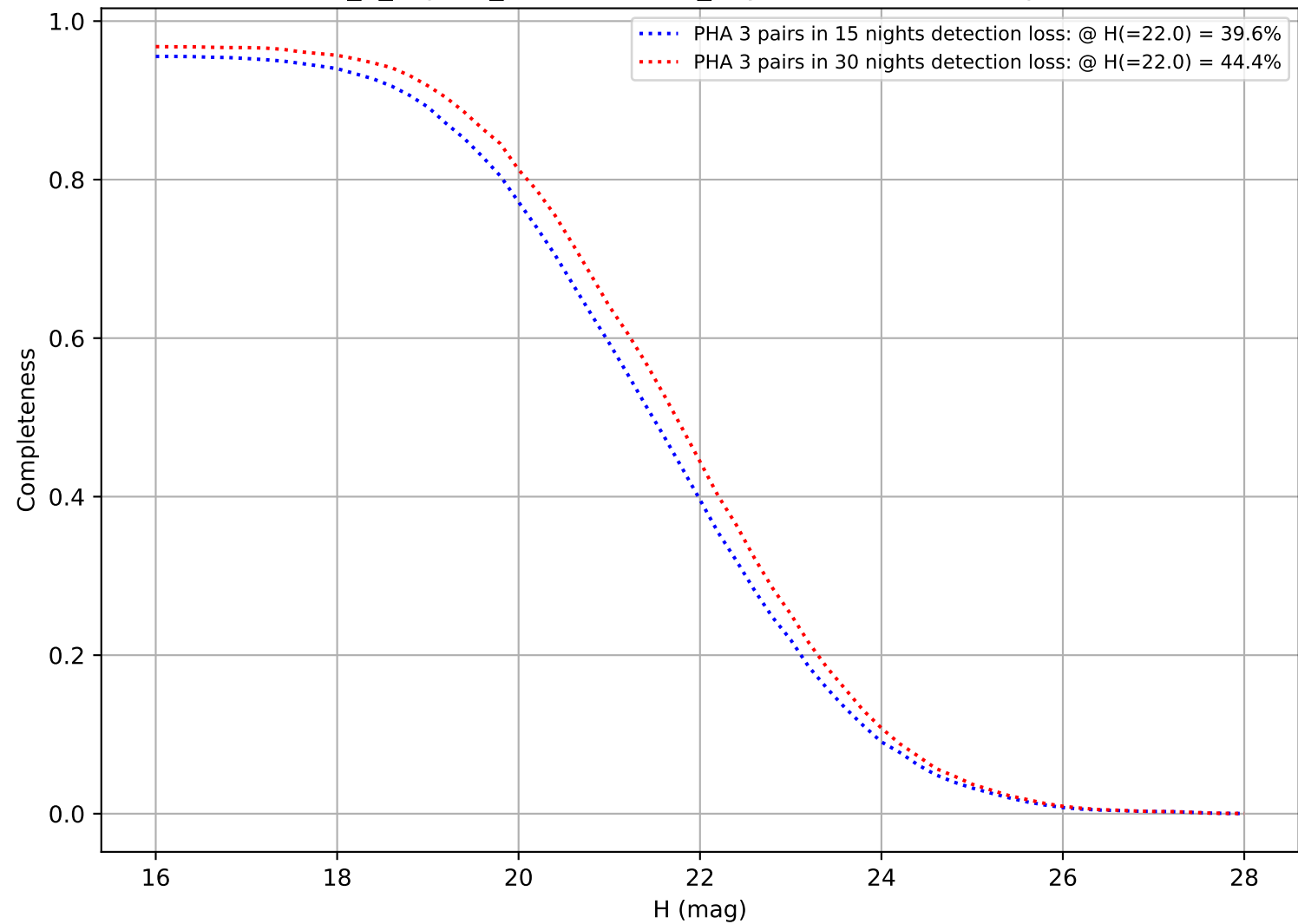
internal_u_expt38_nscale1.1v3.4_10yrs: DifferentialCompleteness
