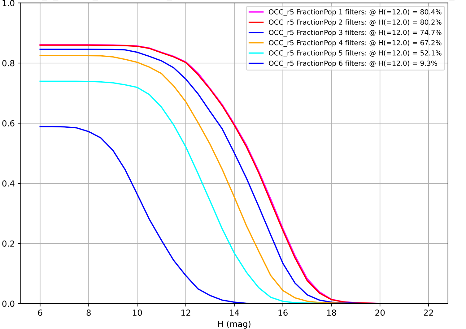
internal_u_expt38_nscale1.1v3.4_10yrs: Fraction of population with colors in X filters OCC_r5
