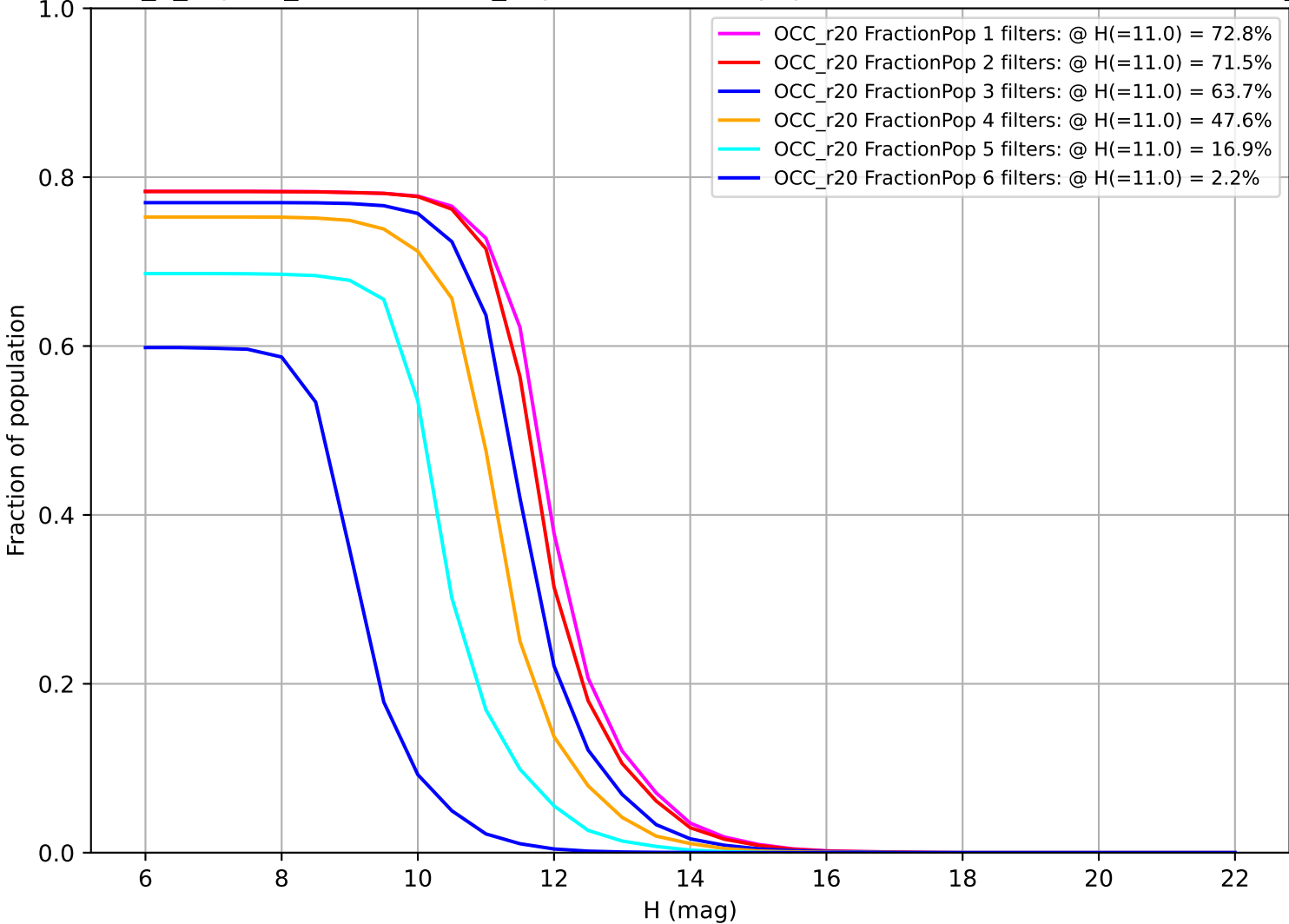
internal_u_expt38_nscale1.1v3.4_10yrs: Fraction of population with colors in X filters OCC_r20
