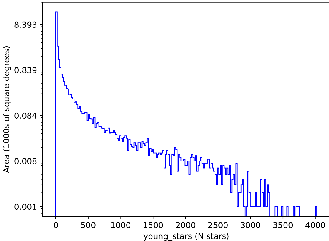
internal_u_expt38_nscale1.1v3.4_10yrs : young_stars
