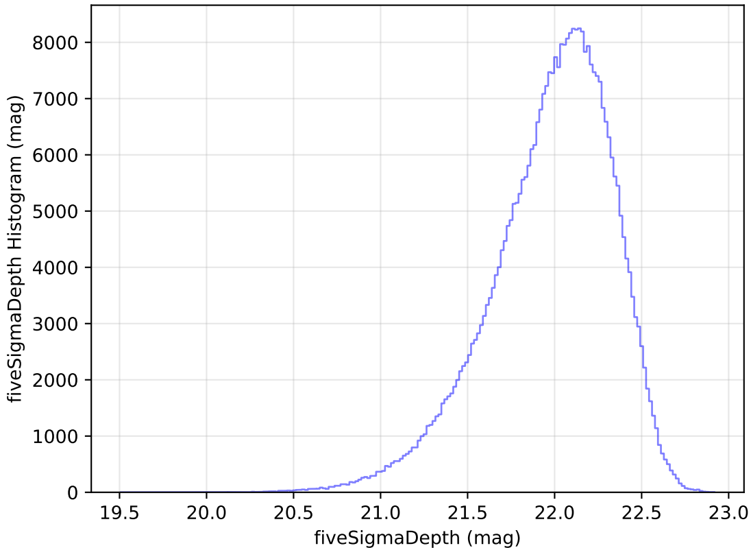
internal_u_expt38_nscale1.1v3.4_10yrs y: fiveSigmaDepth Histogram
