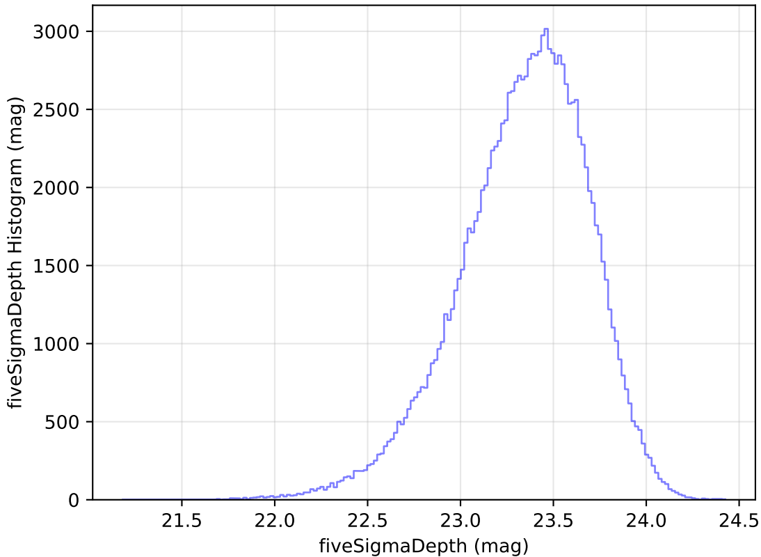
internal_u_expt38_nscale1.1v3.4_10yrs u: fiveSigmaDepth Histogram
