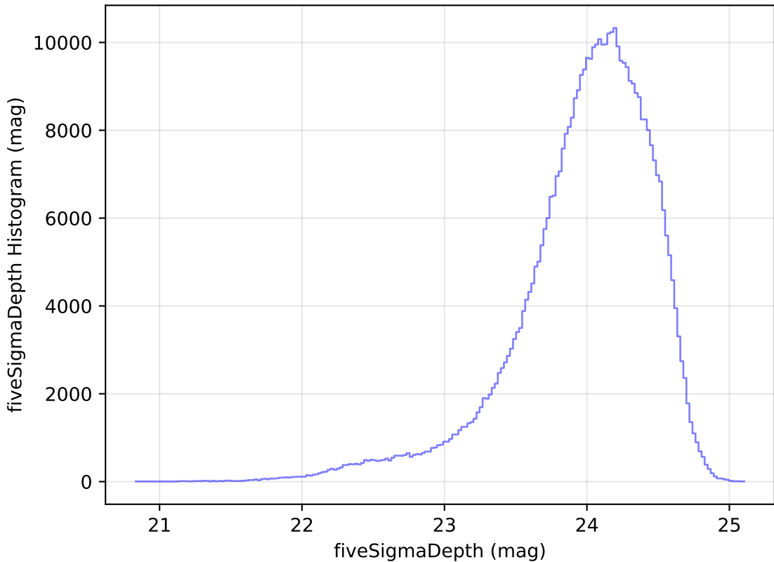
internal_u_expt38_nscale1.1v3.4_10yrs r: fiveSigmaDepth Histogram
