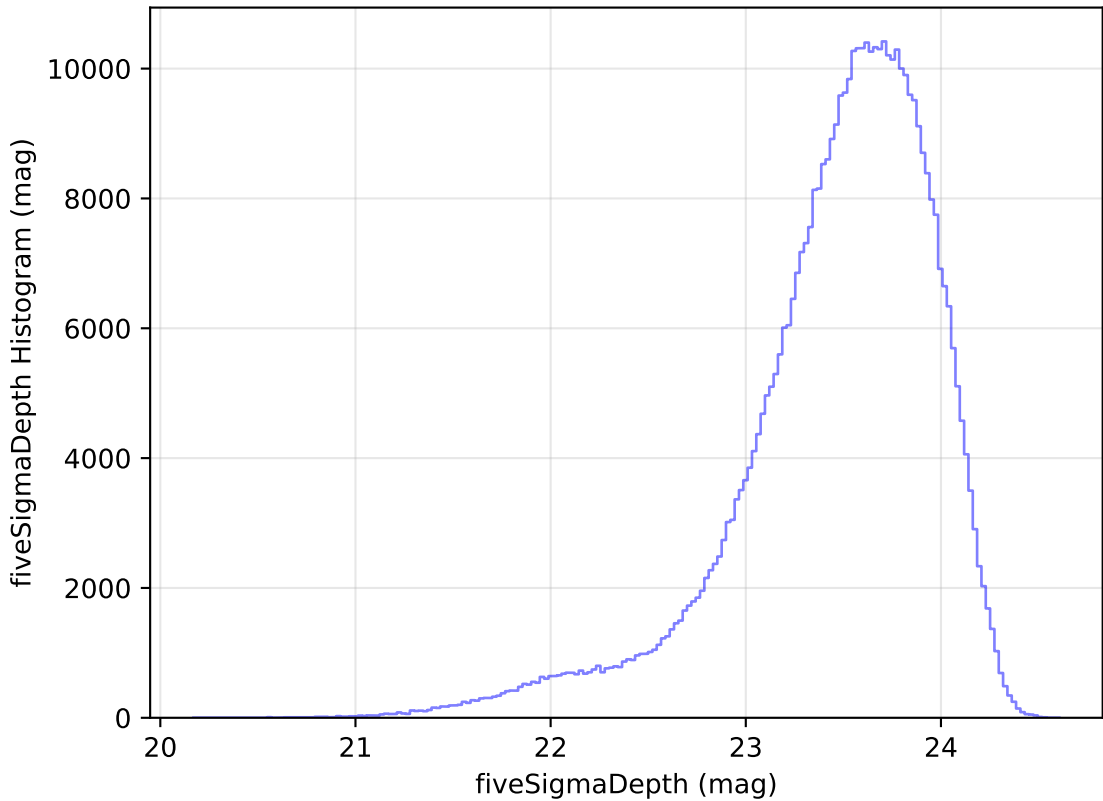
internal_u_expt38_nscale1.1v3.4_10yrs i: fiveSigmaDepth Histogram
