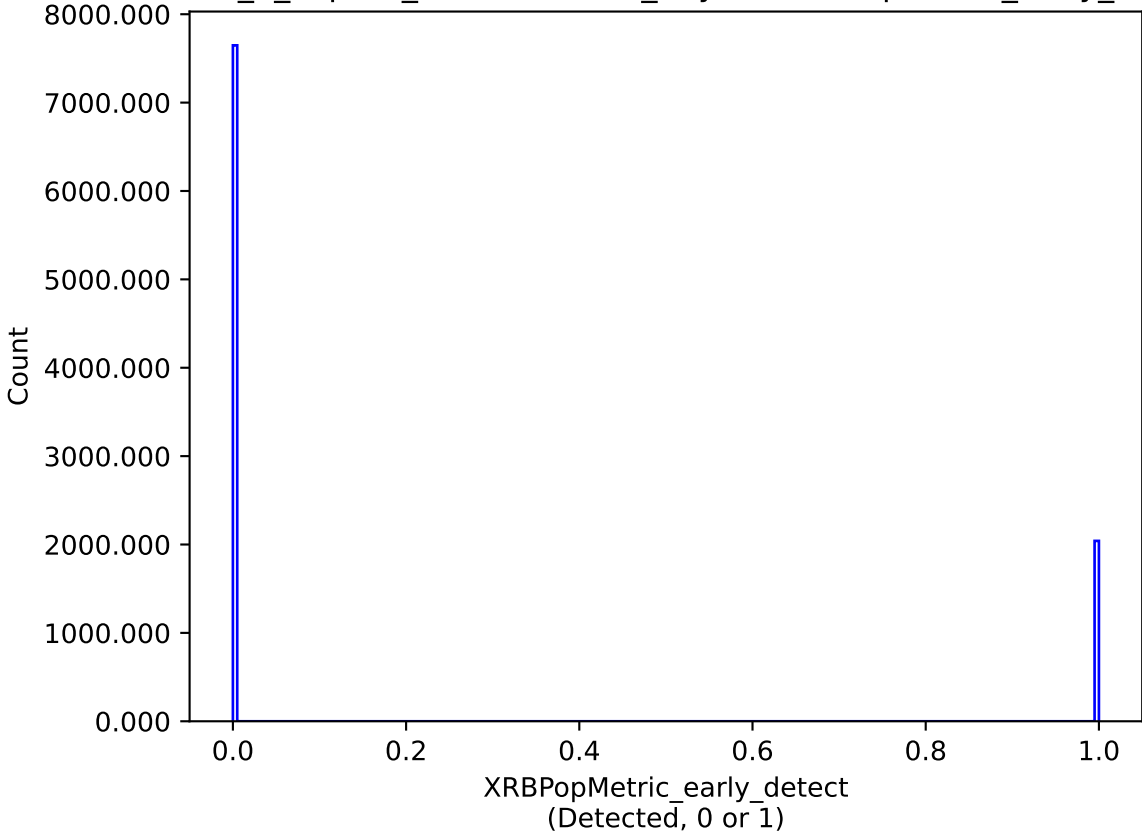
internal_u_expt38_nscale1.1v3.4_10yrs : XRBPoMetric_early_detect
