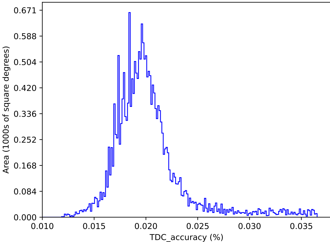
internal_u_expt38_nscale1.1v3.4_10yrs : TDC_accuracy
