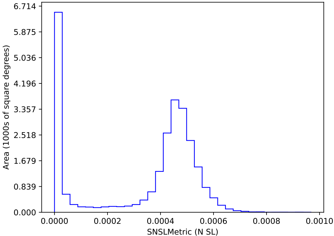
internal_u_expt38_nscale1.1v3.4_10yrs : SNSLMetric
