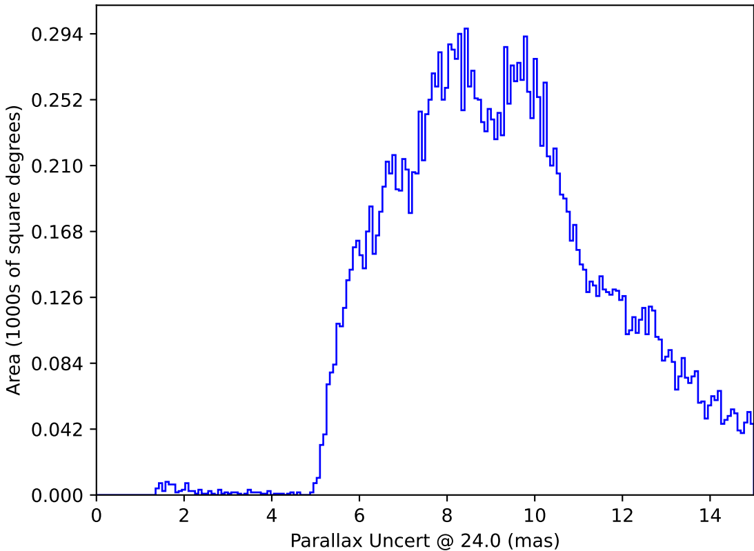
internal_u_expt38_nscale1.1v3.4_10yrs : Parallax Uncert @ 24.0
