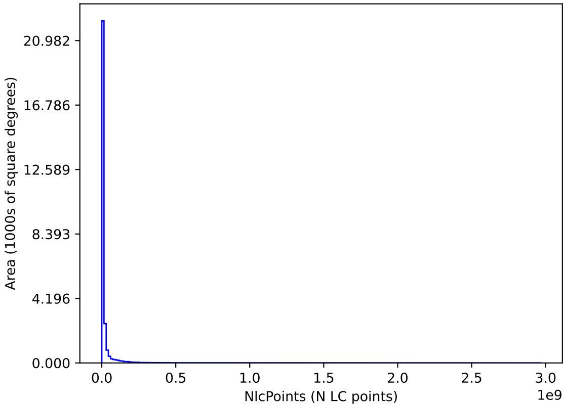
internal_u_expt38_nscale1.1v3.4_10yrs : NlcPoints
