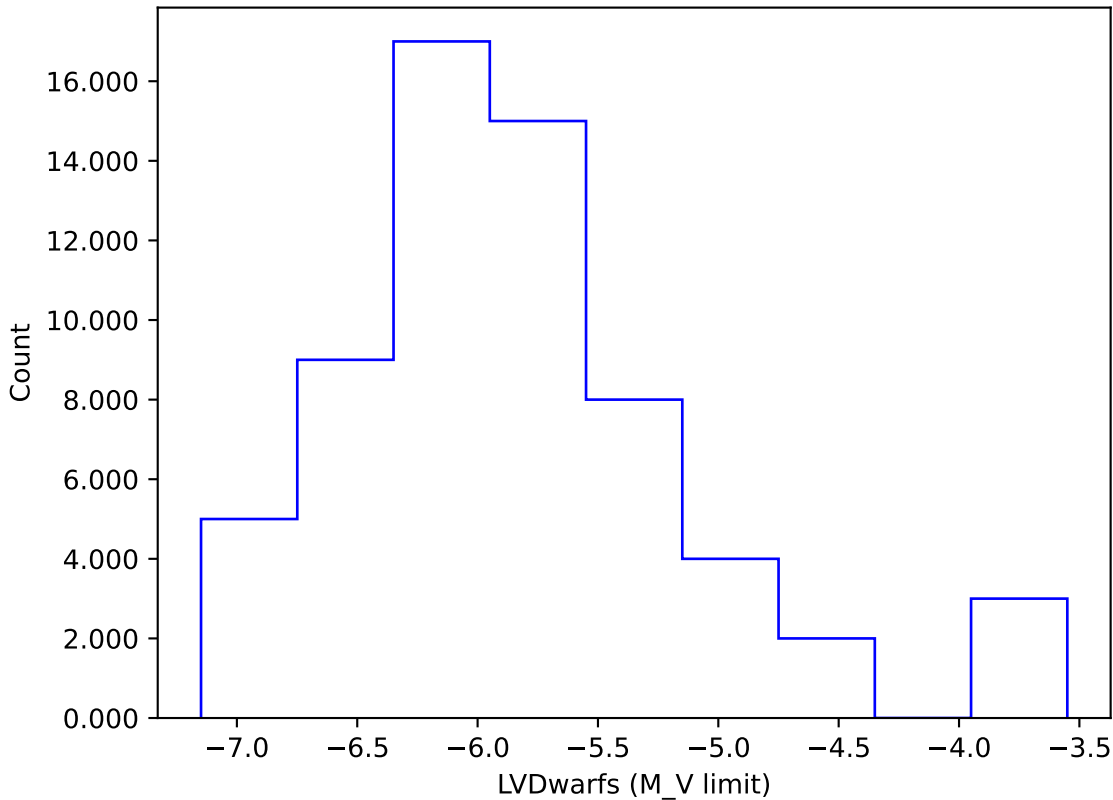
internal_u_expt38_nscale1.1v3.4_10yrs gi: LVDwarfs
