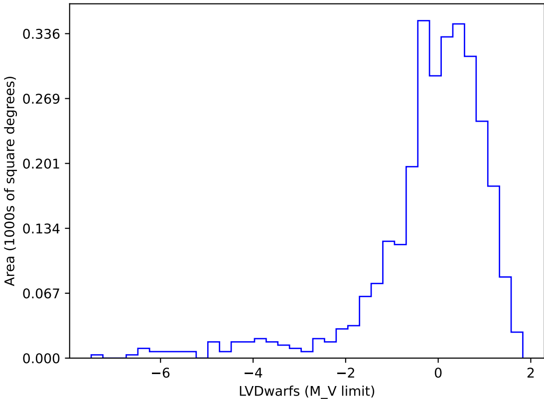
internal_u_expt38_nscale1.1v3.4_10yrs gi SCP: LVDwarfs
