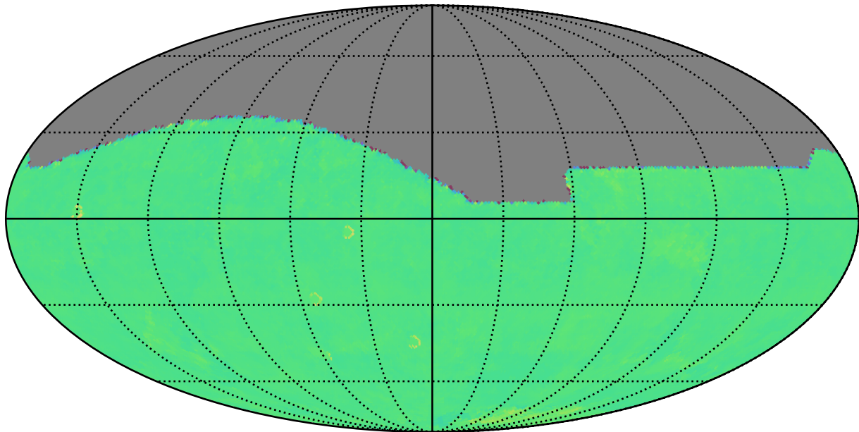
internal_u_expt38_nscale1.1v3.4_10yrs r: Kuiper rotTelPos
