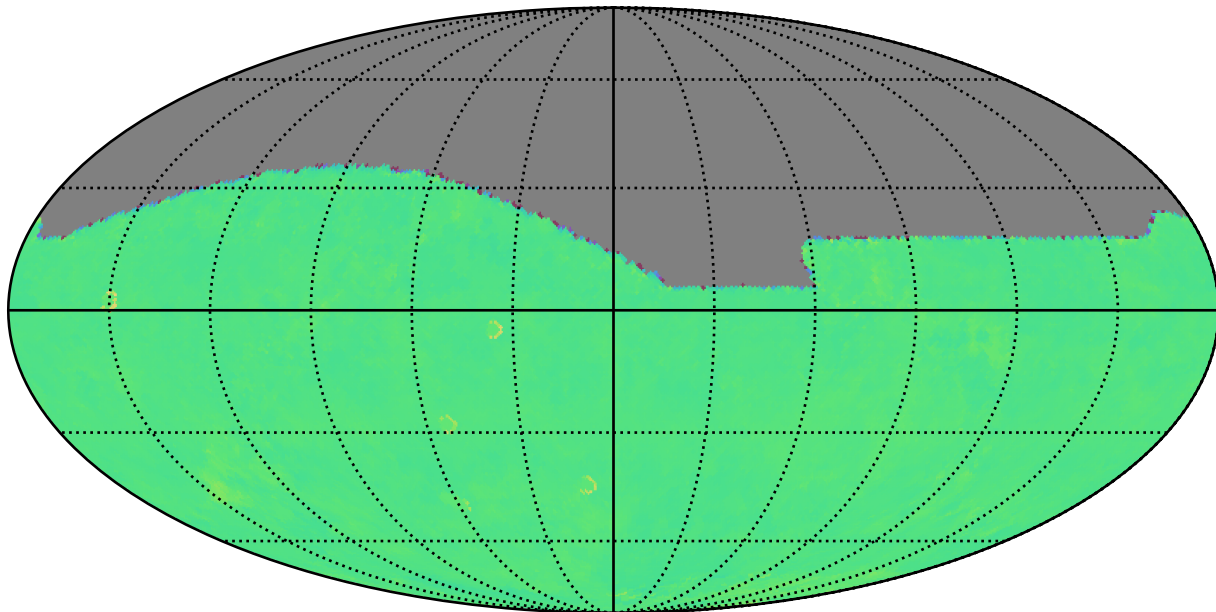
internal_u_expt38_nscale1.1v3.4_10yrs i: Kuiper rotTelPos
