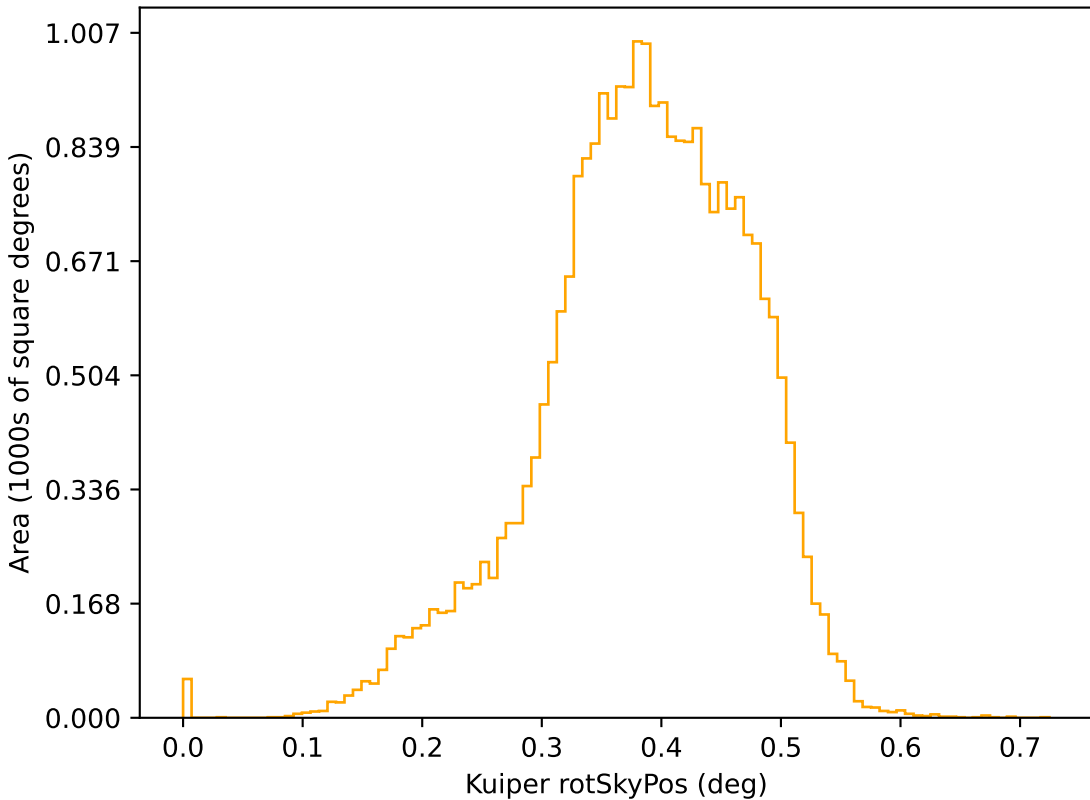
internal_u_expt38_nscale1.1v3.4_10yrs r: Kuiper rotSkyPos
